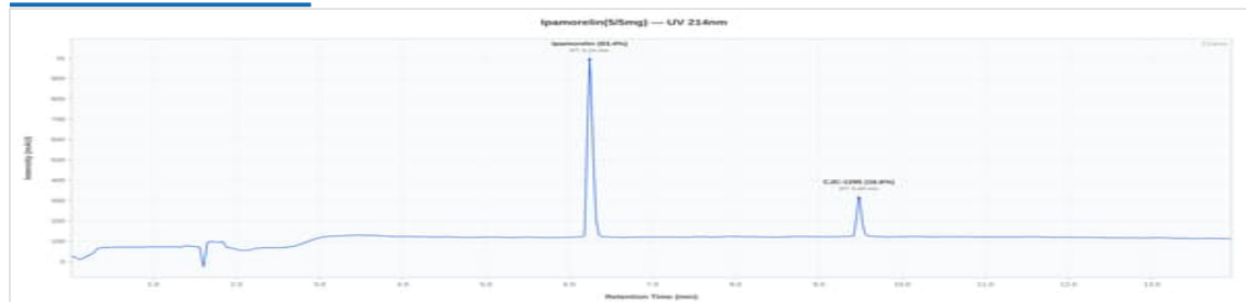
CJC/IPA 5/5mg - CJC0123-03: UV Chromatogram
